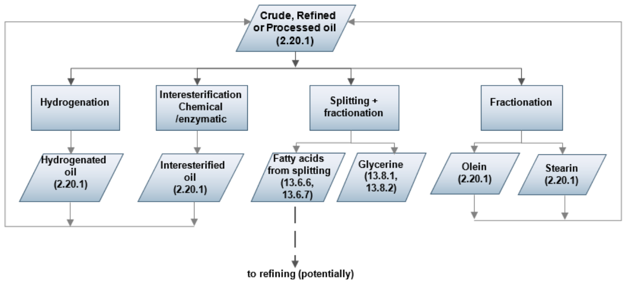
Flow chart downstream processing
